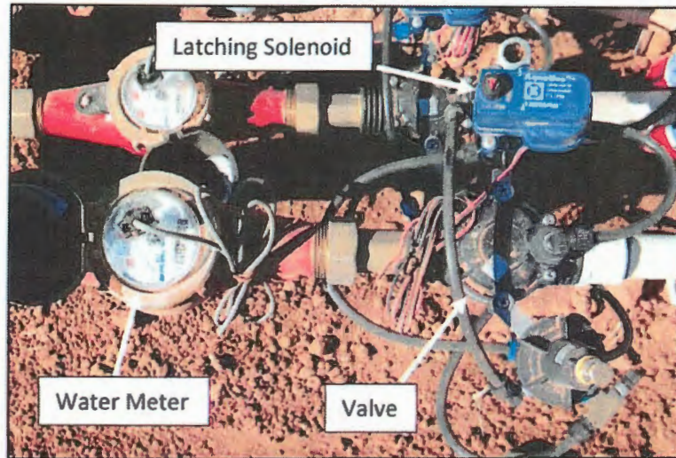
Figure 2. Flow meter, water control valve and latching solenoid valve used at valve control stations supplying water to each of 47 SDI zones, Texas A&M AgriLife Research, Halfway, TX, 2019.
